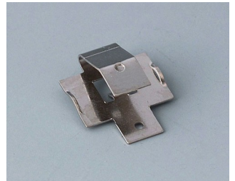
A9193009 Battery clips, single contact CuBe nickel-plated
