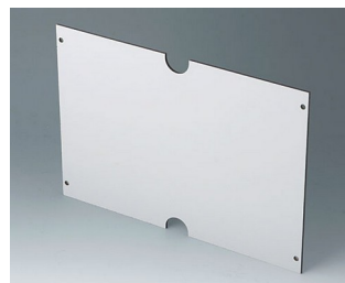
C7117056 Mounting plate 220.5x152.5x2.5mm
