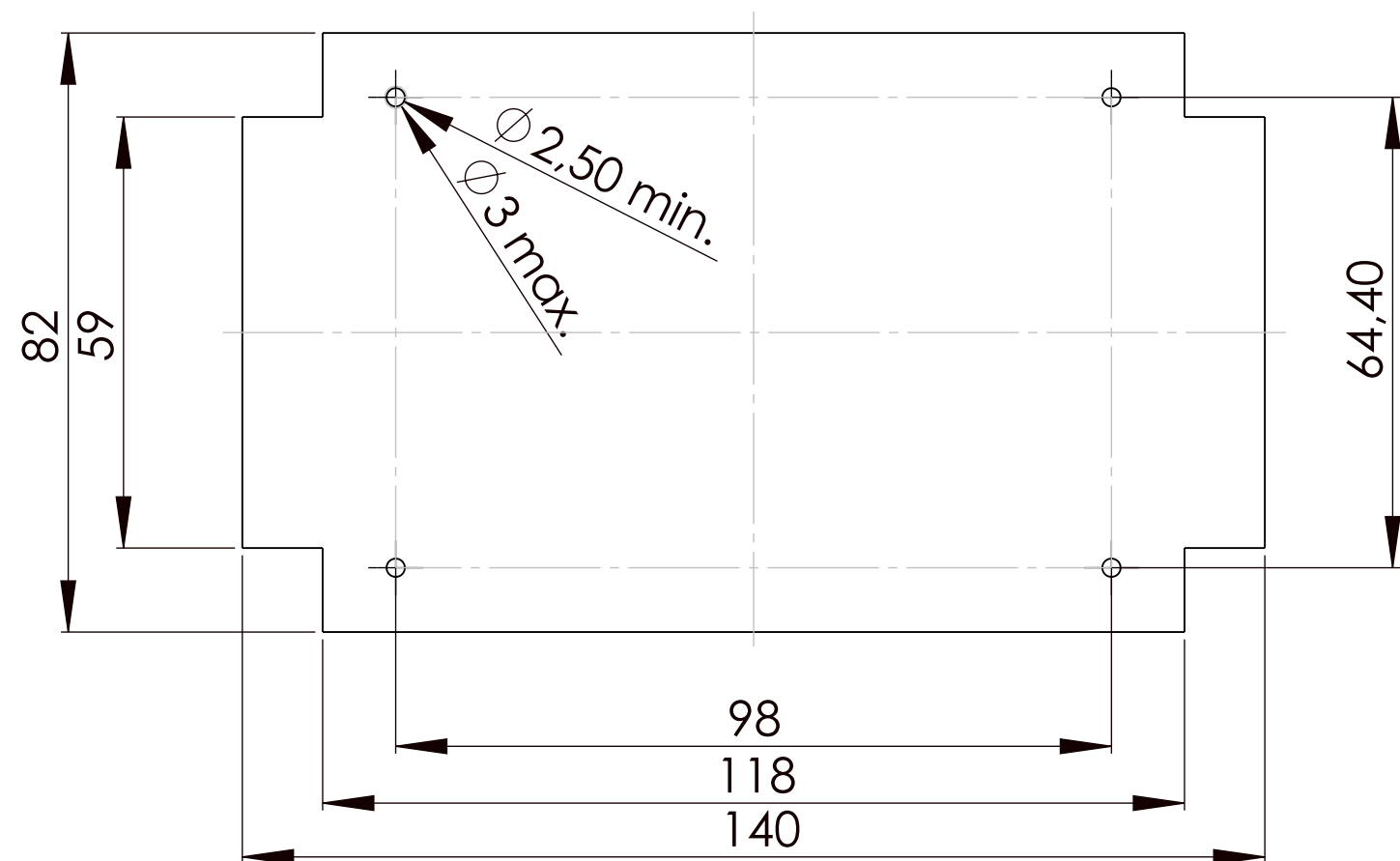
Platine OT P C B
