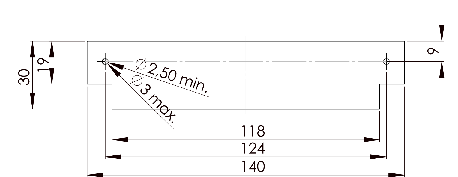
Platine UT Batteriefach P C B battery-compartment
